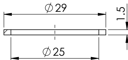
SECTION X-X
