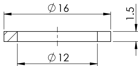
SECTION X-X
