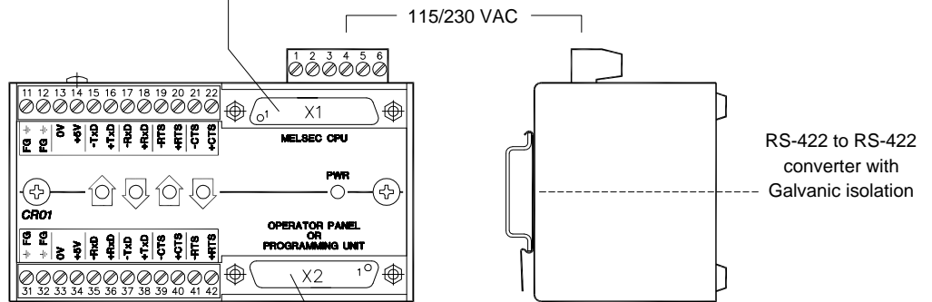
CR-01 Schematic drawing 02203 Outline drawing 02202
