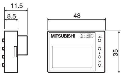
FX3U-7DM
