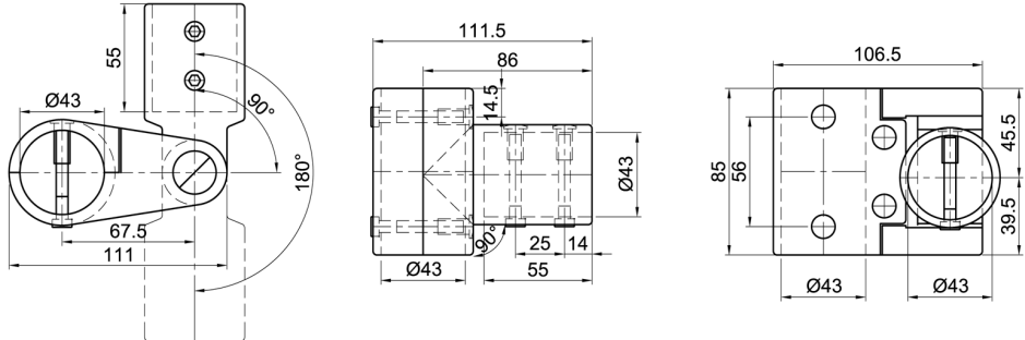
Pendellager 43 x 43 180° Swivel bearing 43 x 43 180°
