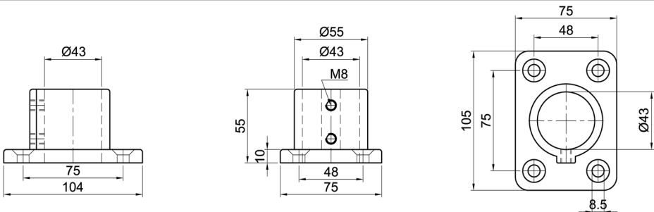
Bodenlager, 1-schalig Ground bearing, 1-shell
