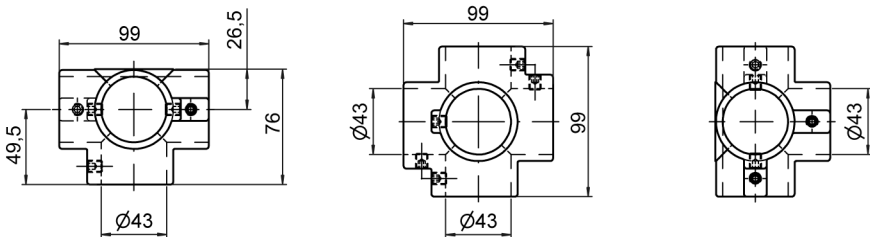
Kreuzverbinder 5-fach, 1-schalig Cross connector 5 end, 1-shell
