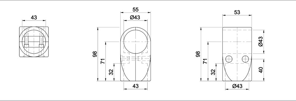
T-Verbinder, 2-schalig T-Connector, 2-shell
