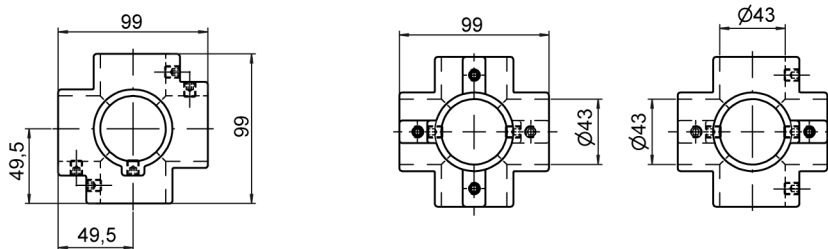
Kreuzverbinder 6-fach, 1-schalig Cross connector 6 end, 1-shell
