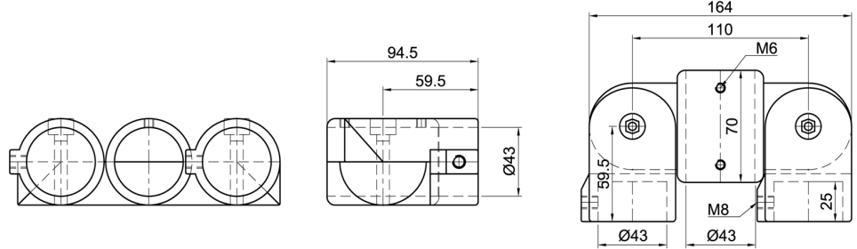
Kreuzverbinder 5-fach, 1-schalig Cross connector 5 end, 1-shell
