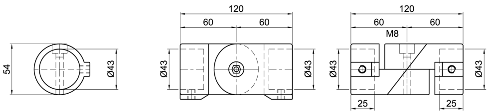
Winkel-Gelenkverbinder, 1-schalig Angle joint connector, 1-shell
