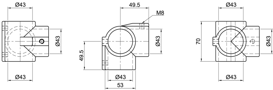
Eck-Verbinder 90°, offen, 1-schalig Corner connector 90°, open, 1-shell
