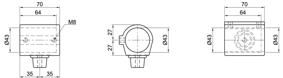
Rohrhalter-S, Kopfstück, 1-schalig Tube holder-S, headpiece, 1-shell
