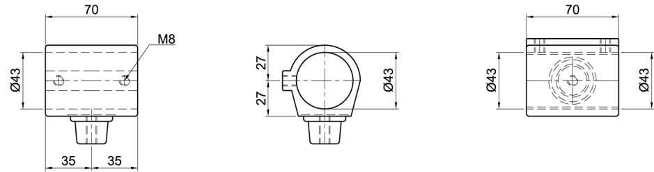
Rohrhalter-S, 1-schalig Tube holder-S, 1-shell
