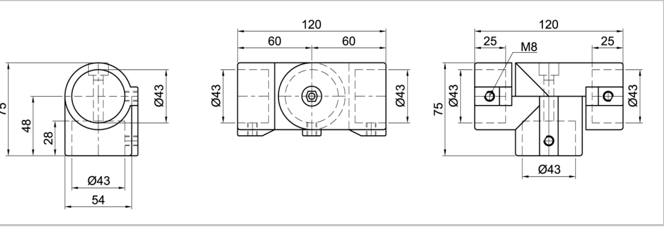
T-Gelenkverbinder, 2-schalig Cross-joint connector, 2-shell
