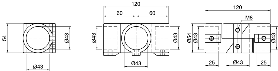
Kreuz-Gelenkverbinder, 1-schalig Cross- joint connector, 1-shell
